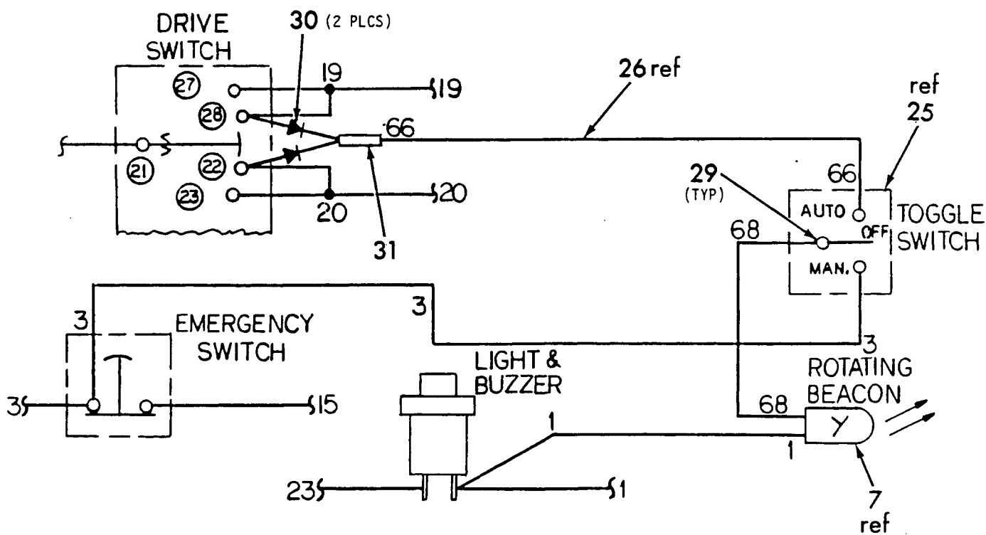
WIRING DIAGRAM
