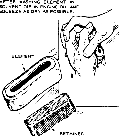
AIR CLEANER
