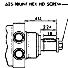
STRAIGHT KEY
