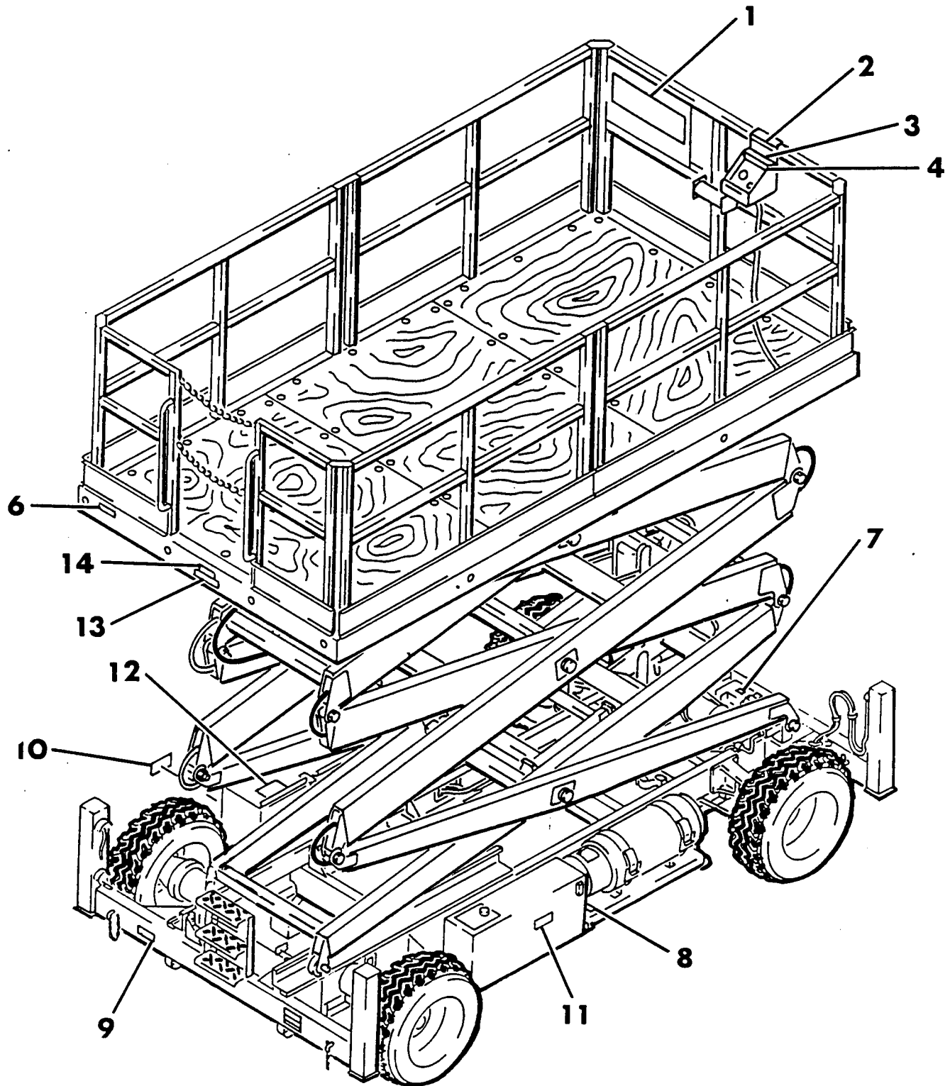
SHOWN MODEL RT-31G
