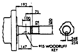
*WOODRUFF KEY
