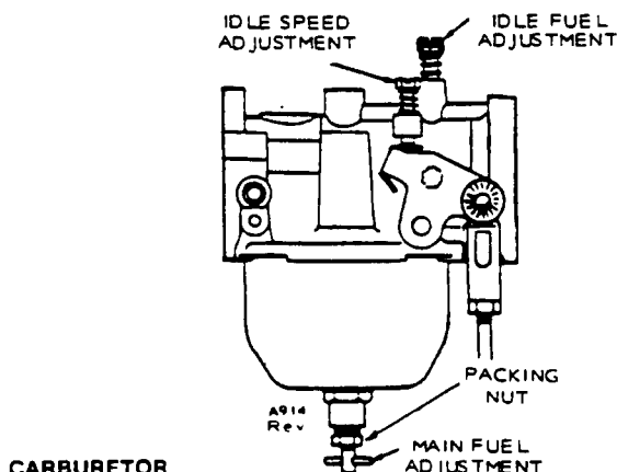
CARBURETOR ADJUSTMENTS
