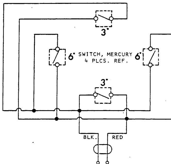
WIRING DIAGRAM
