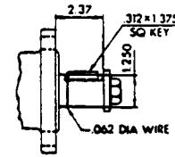
STRAIGHT KEY
