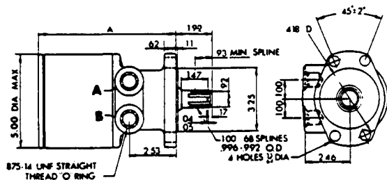
*6-B SHAFT (SAE J499 STANDARD)
