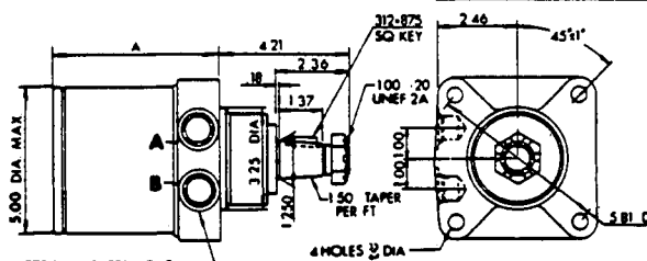
TAPERED SHAFT (SAE J501 STANDARD)
