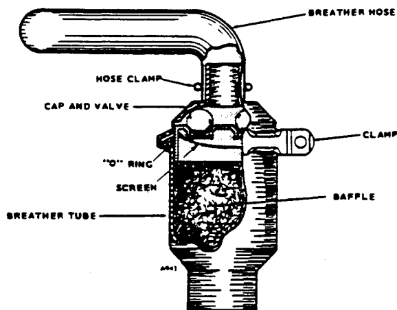
CRANKCASE BREATHER
