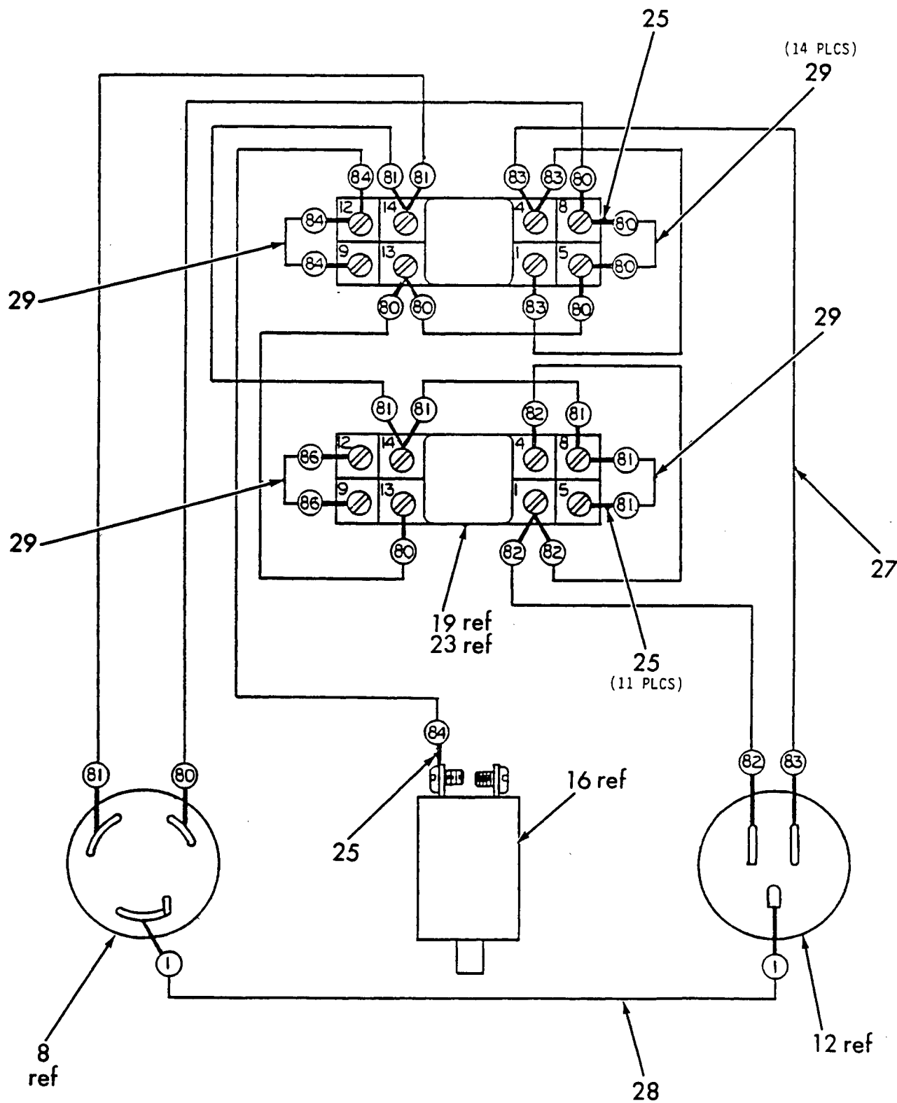
WIRING DIAGRAM
