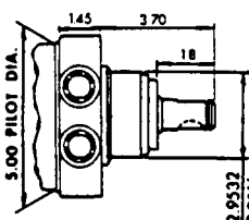
*WOODRUFF KEY
